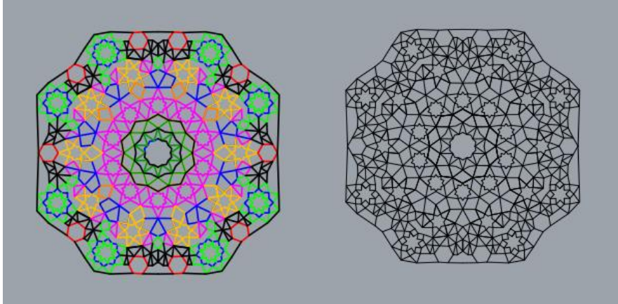
Figure 13: Plan scheme in which the geometries of the muqarnas of the Sahip Ata mosque are determined.
