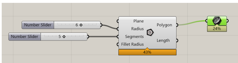
Figure 12: Connecting the " Curve " component to " Polygon "
