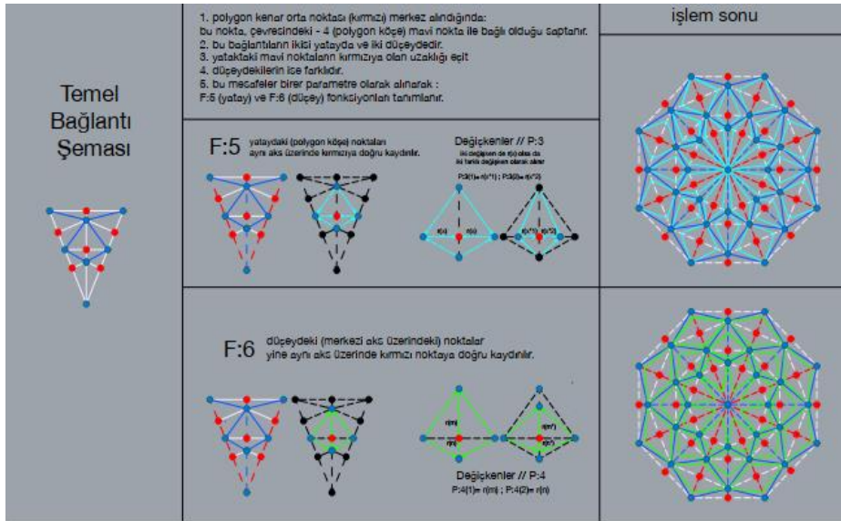
Figure 19: Determination of points and symmetry and view of point coordinates in the basic connection diagram of the main muqarnas of the study on the Grasshopper program
